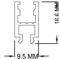
SPACER PROFILE CAT. NO.: 309
