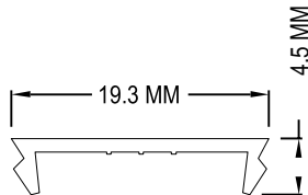
SCREW COVER PROFILE CAT. NO.: 308
