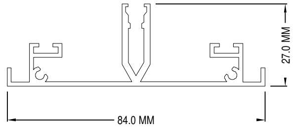
BASE PROFILE CAT. NO.: 307
