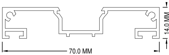
CAP PROFILE CAT. NO.: 306
