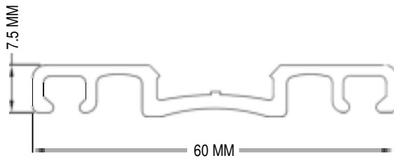
PRESSURE PROFILE (CAP PROFILE 352)
