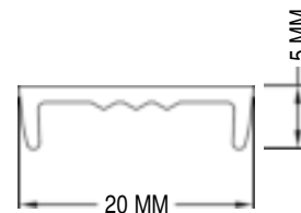
CAP COVER 308
