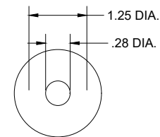
⑦ 1/4" WASHER (1/16" THICK)
