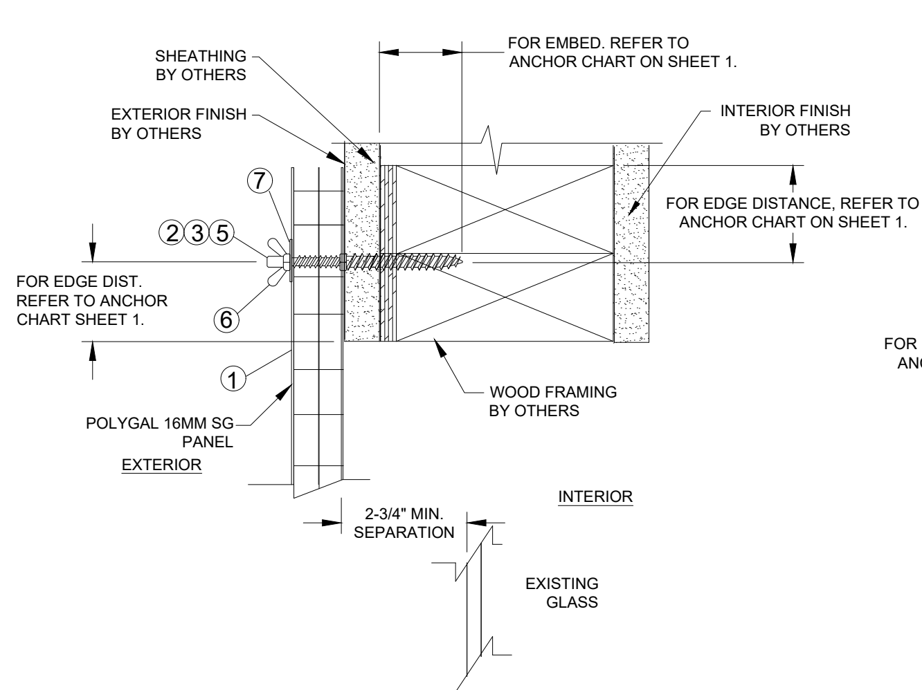
A 3 VERTICAL SECTION WOOD FRAME SUBSTRATE WALL MOUNT INSTALLATION
