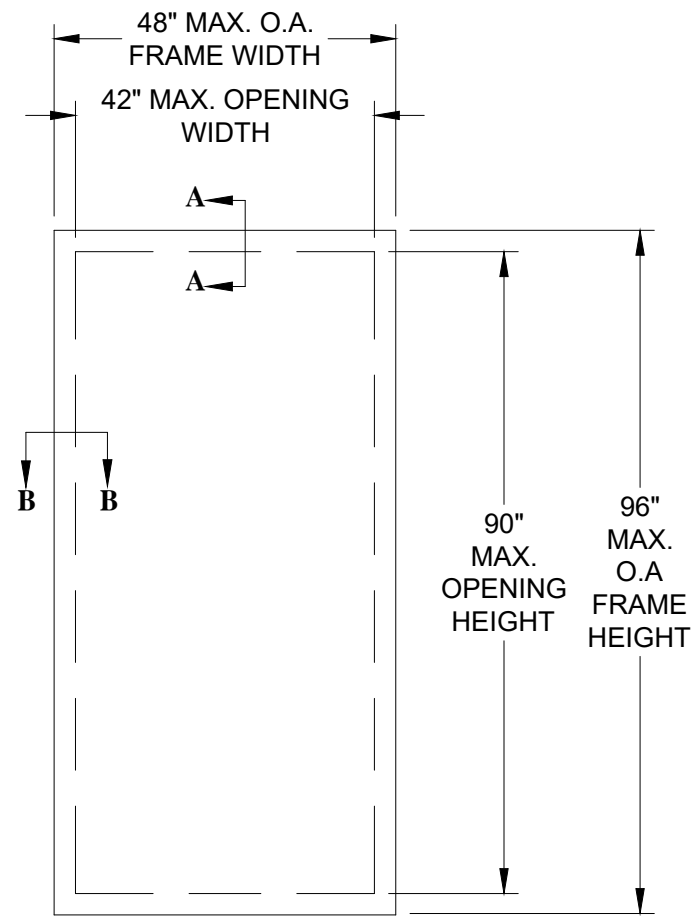
ELEVATION POLYGAL SG 16MM EXTERIOR VIEW
