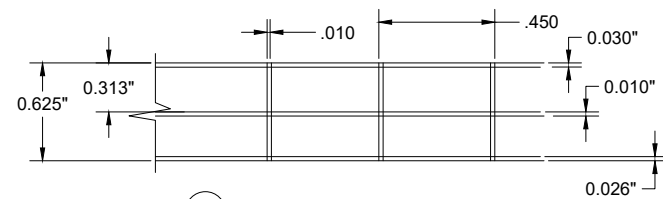
① POLYGAL 16MM PANEL CROSS SECTION POLYCARBONATE
