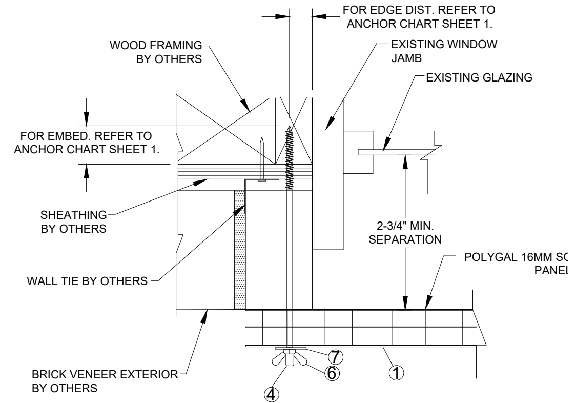
B 5 HORIZONTAL SECTION SOLID BRICK VENEER ANCHORING WALL MOUNT INSTALLATION
