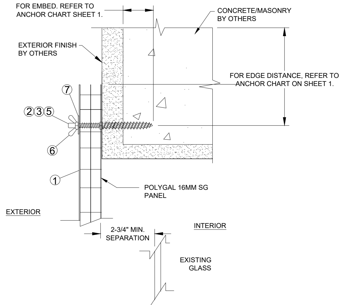
A 4 VERTICAL SECTION CONCRETE SUBSTRATE WALL MOUNT INSTALLATION
